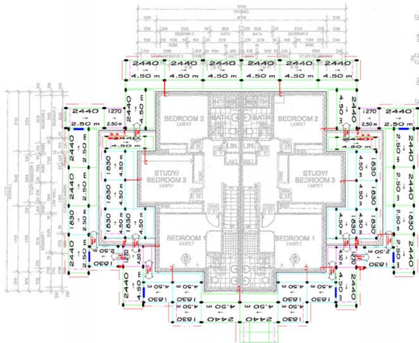
PLAN VIEW
